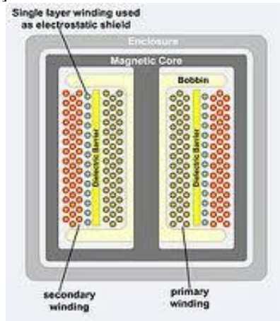
Fig.2 isolation transformer
