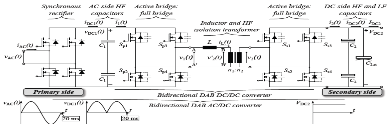
Fig.1 Bidirectional Dual Active Bridge AC/DC converter Topology
