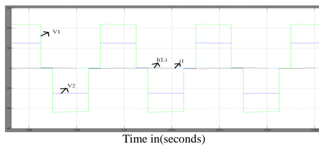
Figure.10 shows the simulated inductor current( I(L) ),primary and secondary side voltages( v1 & v2 ),input DC current( i1 ) by connecting scope
