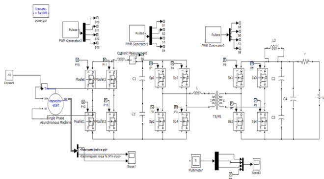
Fig.8 Simulation Diagram of bidirectional AC/DC converter
