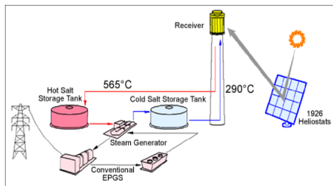
Fig. 2Block Diagram for Solar thermal CSP technology
