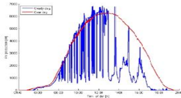
Fig. 4 Example -PV system output on 2 days with passing clouds
