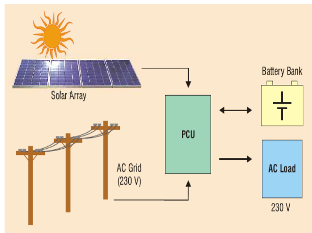
Fig. 1Block Diagram for Solar PV technology
