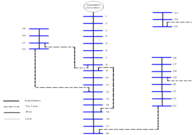
Fig.1:Initial Configuration of the 33 bus radial distribution sytem
