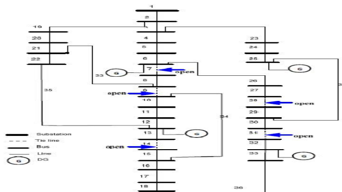
Figure 4. Network Reconfiguration with 4 DGs of 33-bus system
