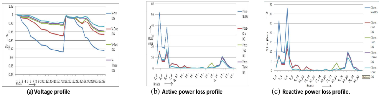
Fig. 3: The Comparative Results for DG installation,
