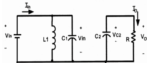
Fig. 4 Mode 1 operation
