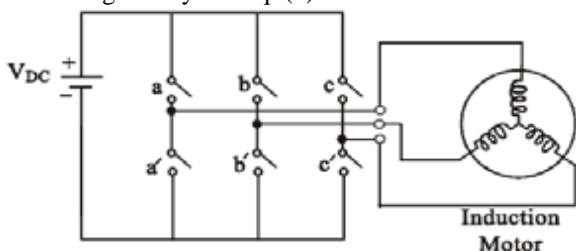
Fig. 1: Power circuit of induction motor
