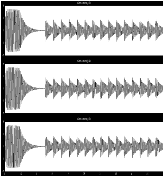
Fig.9 Stator Current of Three phase Induction Motor
