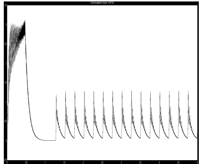
Fig.11 Electromagnetic Torque
