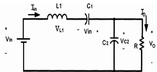
Fig. 5 Mode 2 operation
