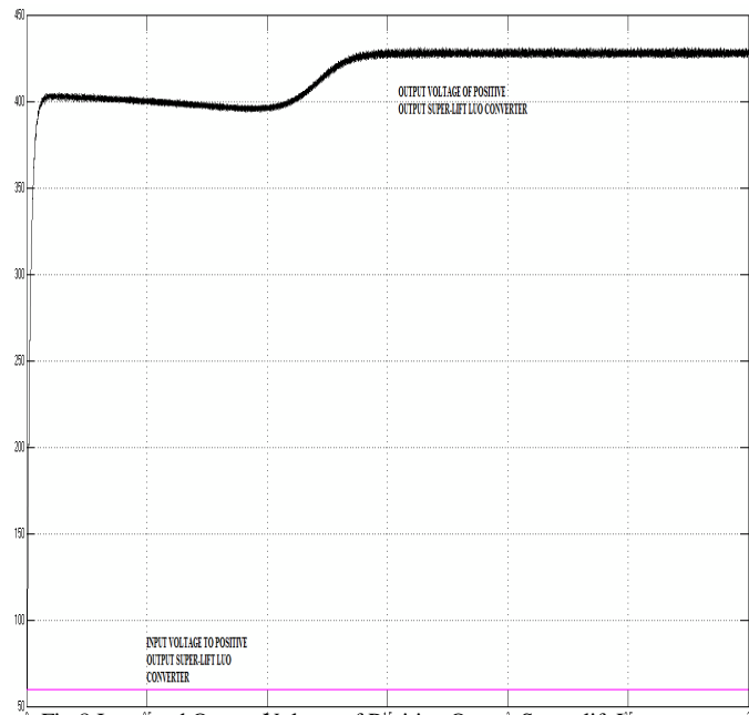
Fig.8 Input and Output Voltage of Positive Output Super-lift Luo Converter
