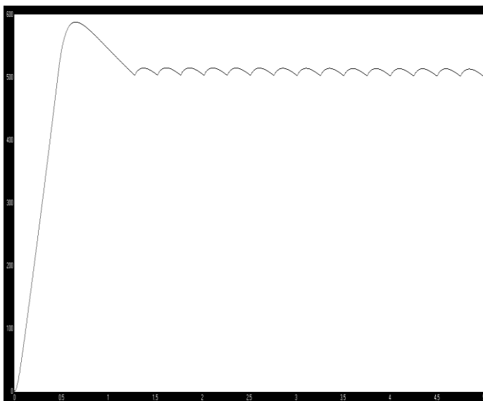
Fig.10 Speed Response of Three phase Induction Motor
