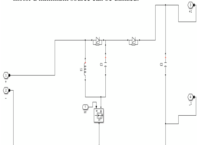
Fig.7 Simulink model of Positive output Super-lift Luo Converter
