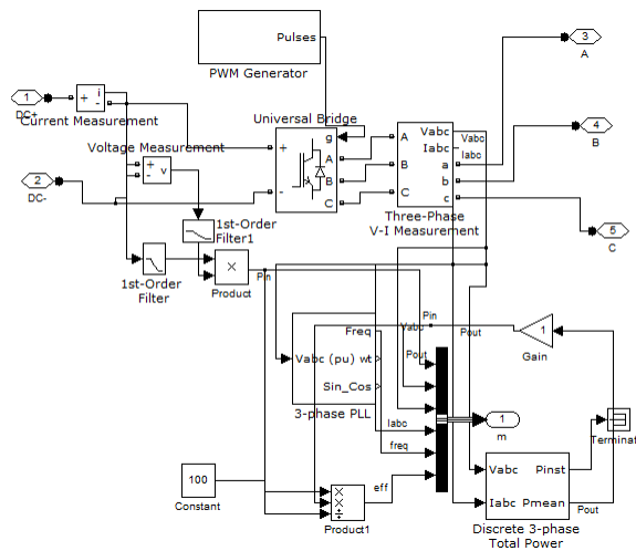
Fig 2. MATLAB/ Simulink model of the inverter circuit.
