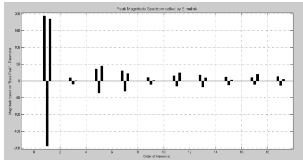
Fig 7(a) THD analysis of the conventional HPS architecture
