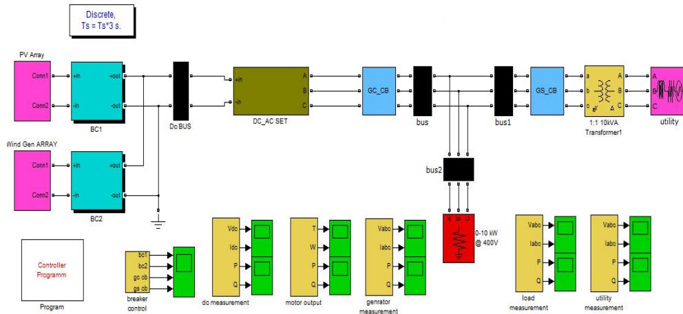
Fig.5 The simulink model of the hybrid power system for energy management and control unit.
