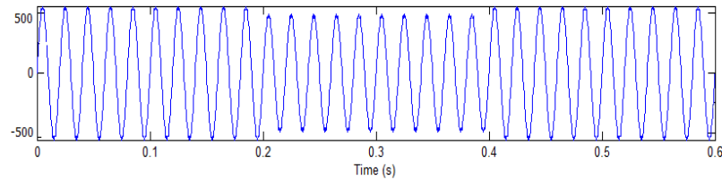
Fig.10 (b) Voltage sag of the MG set under over load condition
