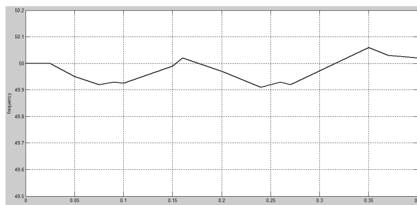
Fig.9 (a) Frequency curve for the inverter
