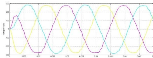
Fig.8(a) The output voltage waveforms of the inverter
