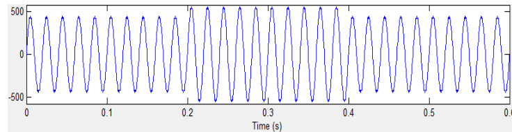
Fig.11(b) voltage swell for MG set under no-load condition.
