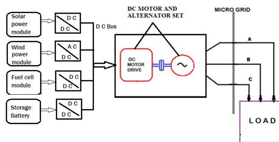
Fig.1 block diagram of the proposed hybrid power system
