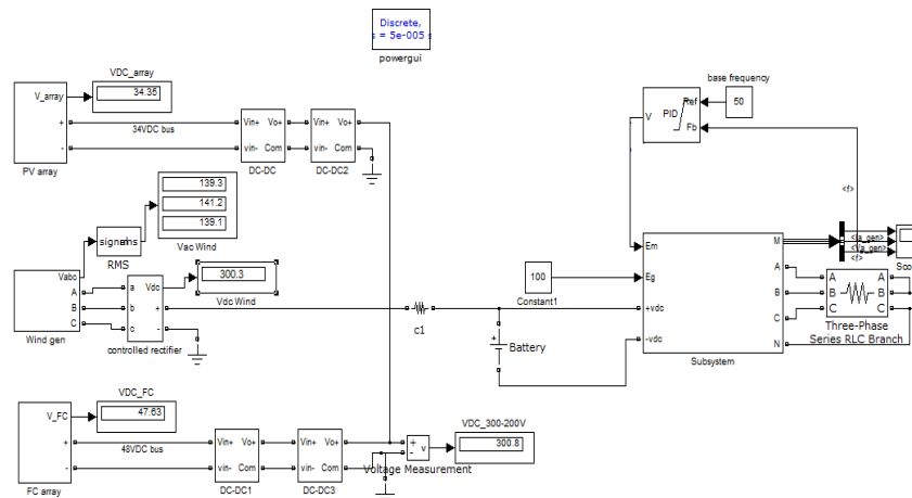
Fig. 4 MATLAB/simulink model of the proposed hybrid power system with dc motor and generator set.
