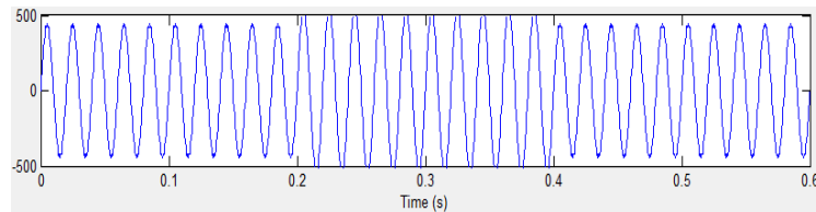
Fig.11(a) voltage swell for inverter model under no-load condition
