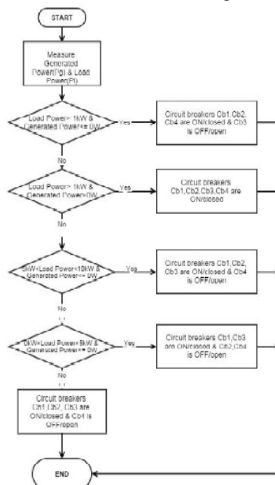
Fig. 6 Proposed algorithm for energy management and control unit.
