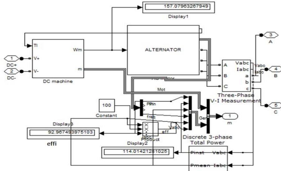
Fig 3. MATLAB/Simulink model of dc motor and synchronous generator set
