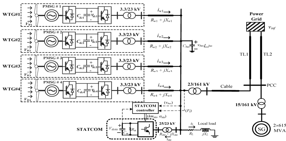
Fig. 1 Configuration of the studied SG-based containing four parallel-operated PMSG-based WTGs with STATCOM
