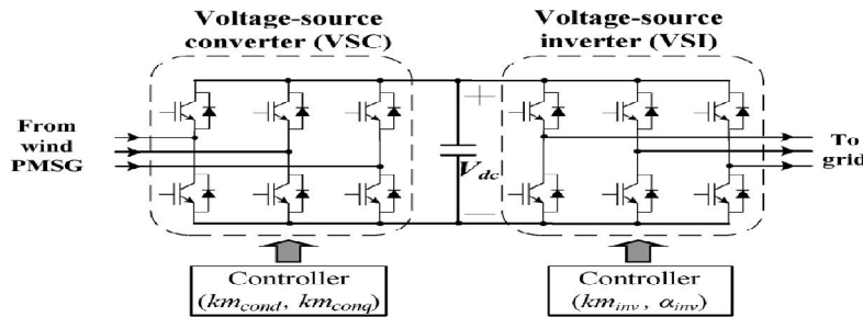
Fig 3 . Model of power converters of the studied wind PMSG
