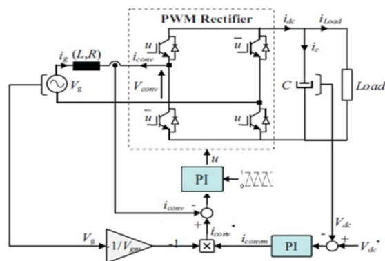
Fig.7.A Closed loop control
