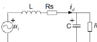
Fig.3 Mode 2/4 operation
