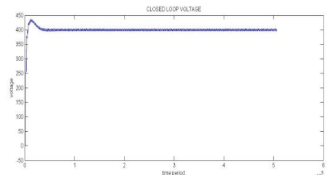
Fig.15. Output voltage for closed loop control
