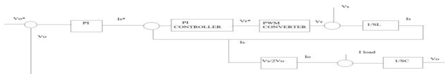
Fig .5. Closed loop block diagram
