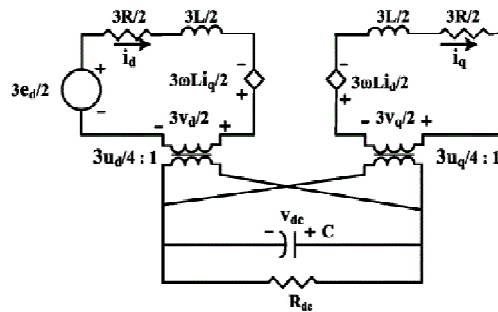
Fig.18. Equivalent circuit in SRF
