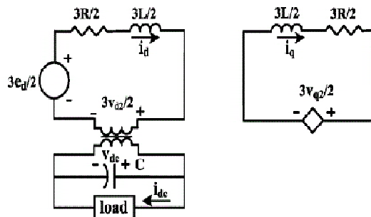
Fig.19. Equivalent circuit in SRF after decoupling q- axis
