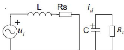
Fig. 2 Mode 1/3 operation
